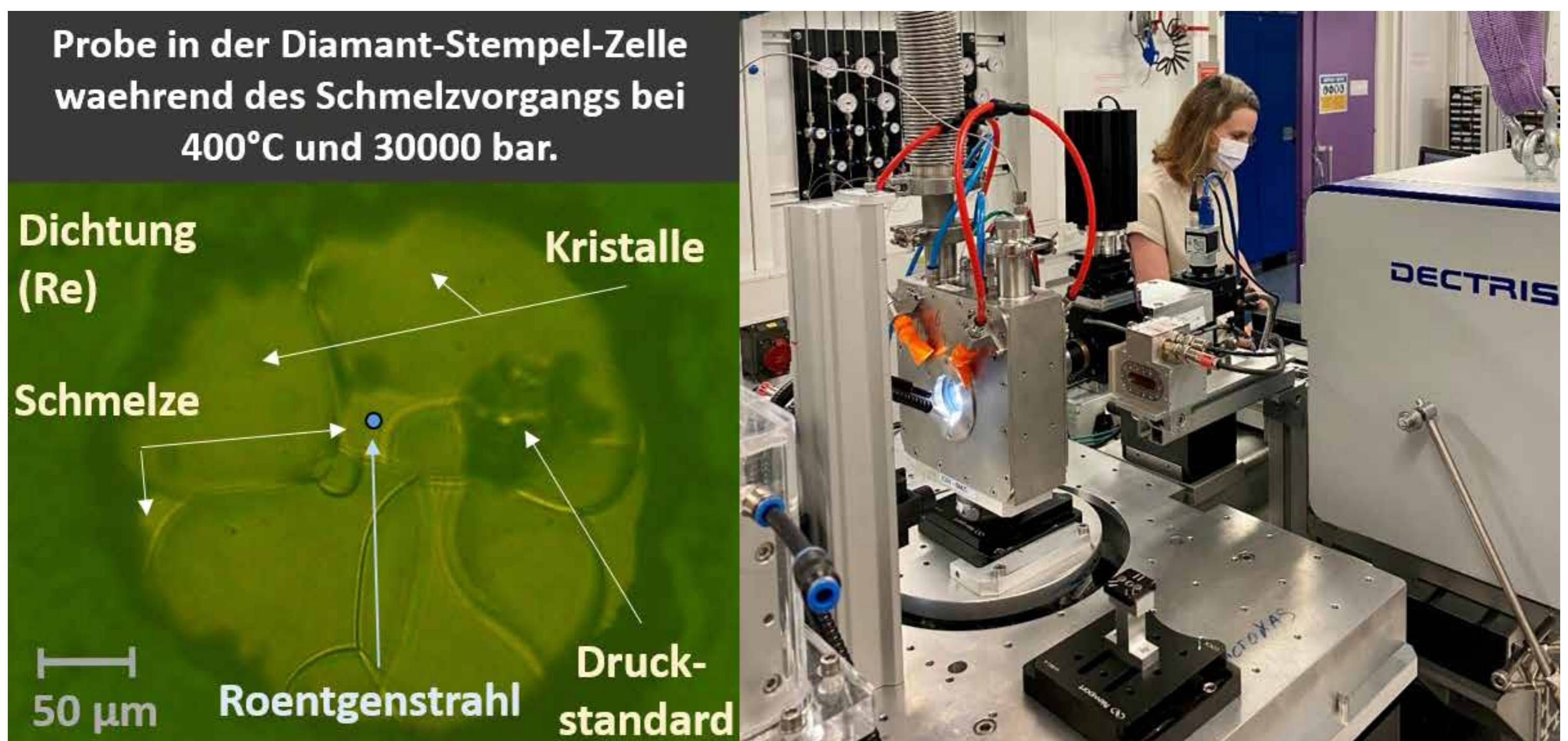
In-situ high pressure and high temperature experiments at synchrotron facilities to study deep planetary interiors. | © Angelika D. Rosa
